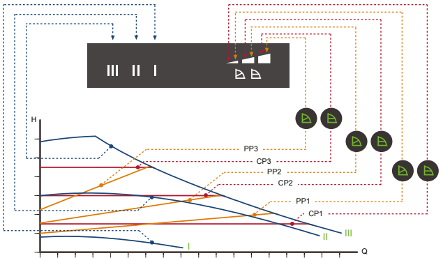
Fig. 1 Pump setting in relation to pump performance
