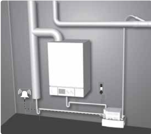
Fig. 12 Installation example
